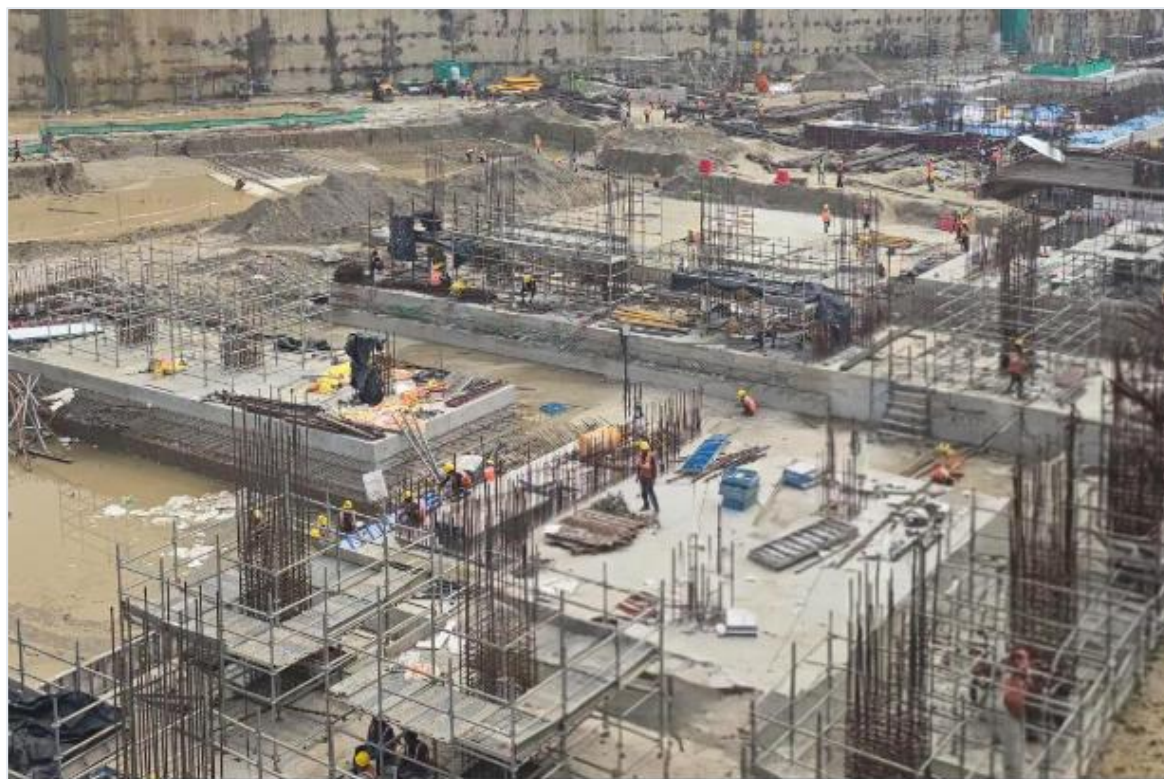
3 Star area — raft and column reinforcement
