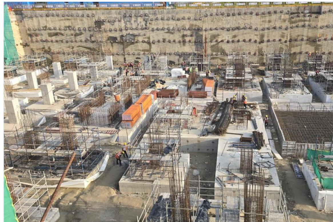
4 Star area — column and pedestal casting
